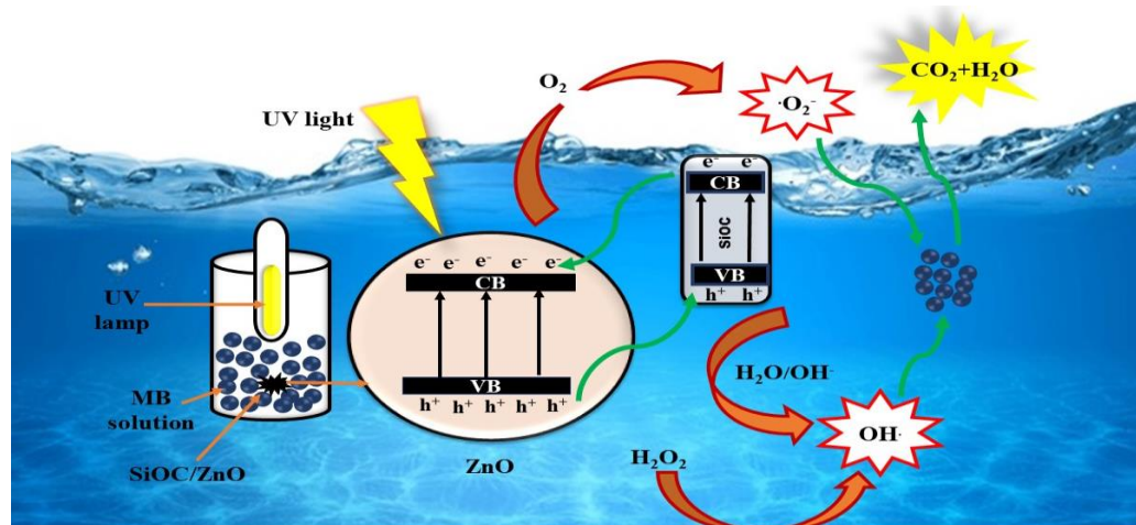
Figure 6. Photodegradation mechanism of methylene blue (MB) under UV light using the SiOC/ZnO composite.
