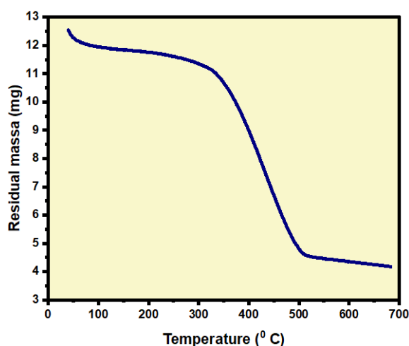
Figure 2. TG curve of vinyl-functional polysiloxane XEN Cure S 32.
