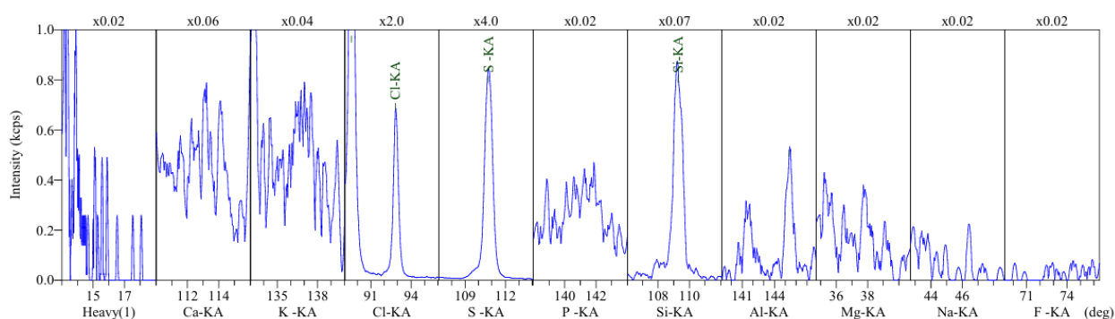
Figure 2. Qualitative XRF analysis chart of the Ferron immobilized PPA fiber
