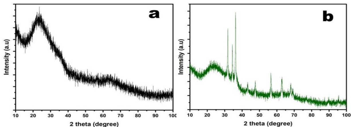
Figure 3. X-ray diffraction (XRD) patterns of (a) SiOC ceramic and (b) SiOC/ZnO composite obtained after pyrolysis at 700 °C.
