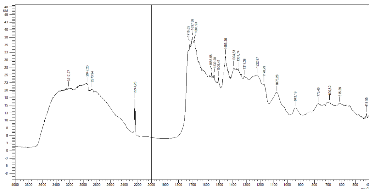
Figure 3. FT-IR spectrum of the polyethylenepolyamine-functionalized polyacrylonitrile (PPA) fiber.
