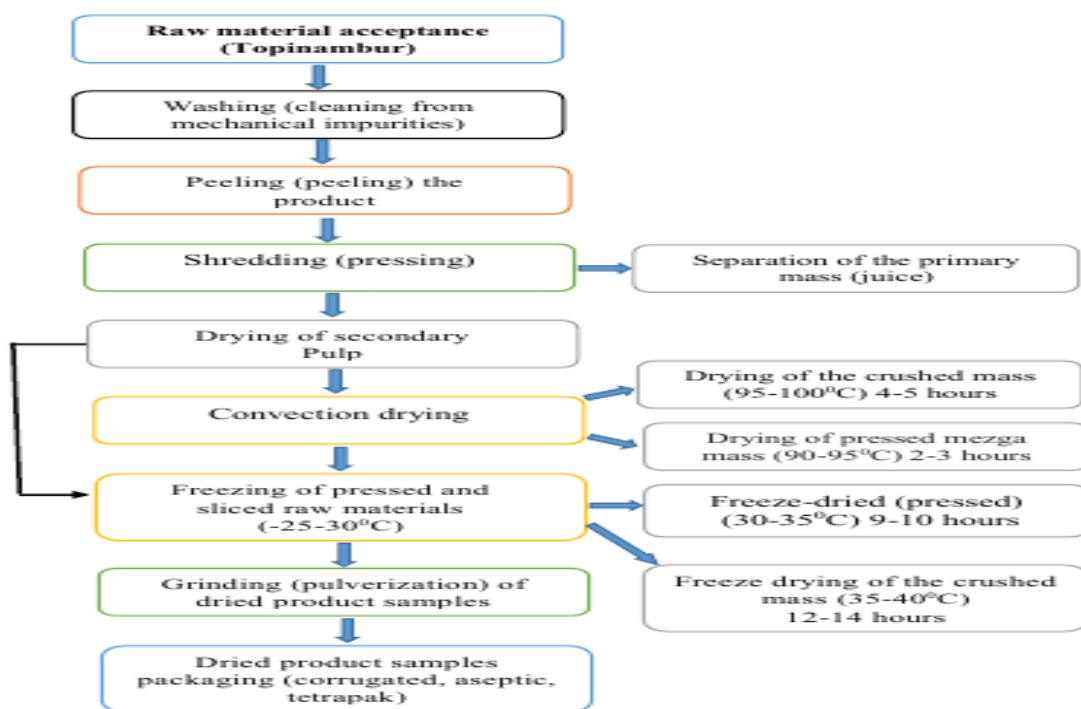
Figure 1. Technological scheme of complex processing of topinambur
