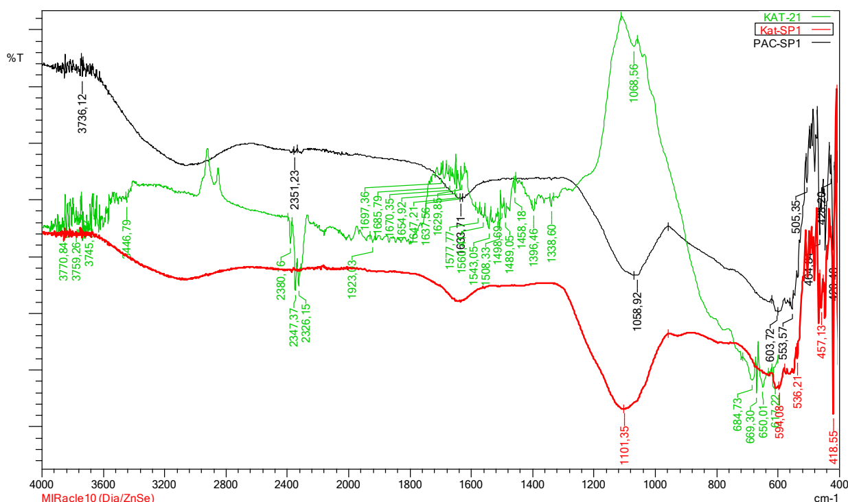
1-rasm. PAC–Cel–P–PAA gibrid koagulyantining FTIR spektri tahlili
