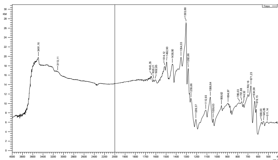
3-rasm. Tiron organik reagentining infraqizil spektr tahlili
