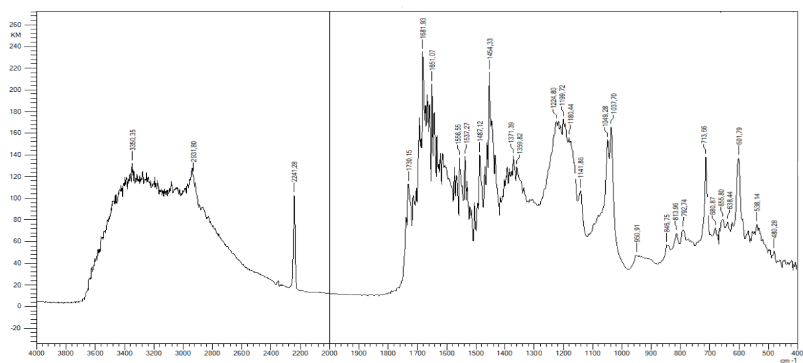
Figure 4. FT-IR spectrum of the PPA fiber after immobilization of the Ferron ligand.
