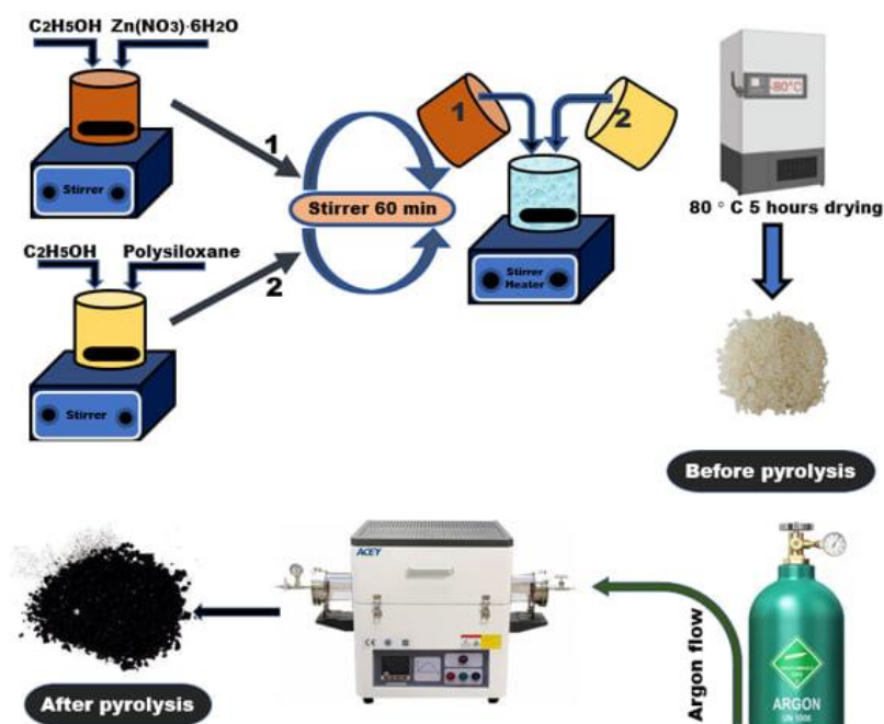
Figure 1. Schematic illustration of the preparation process of the SiOC composite modified with ZnO nanoparticles.
