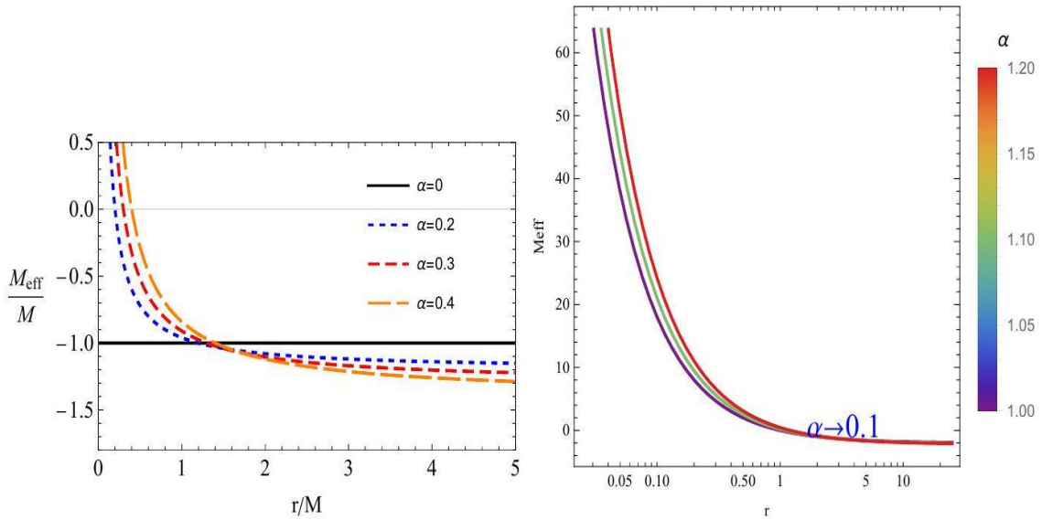
Fig 3: Graphical illustration of effective mass along the radial distance r for different values of the parameters. The black solid line corresponds to the Schwarzschild black hole, while dots on each curve locate the location of the event horizon.
