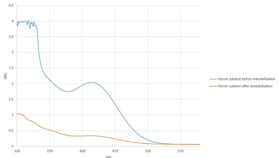
Figure 1. UV-Vis absorption spectra of 20 mL 0.02 M Ferron solution before and after immobilization on PPA fiber, showing characteristic absorption at 434 nm.
