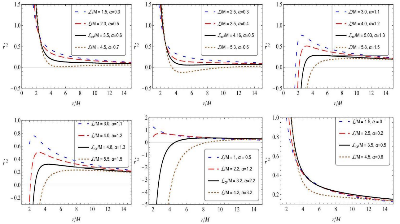
Fig 2: Radial dependence of the square of radial velocity for different values of angular momentum of the particle.
