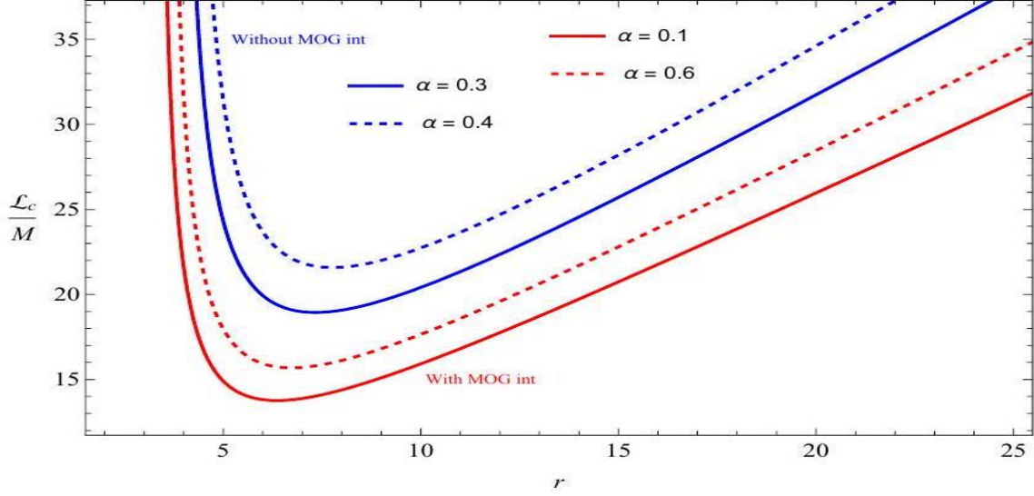
Fig 1: Radial dependence of the critical angular momentum with and without MOG interaction.
