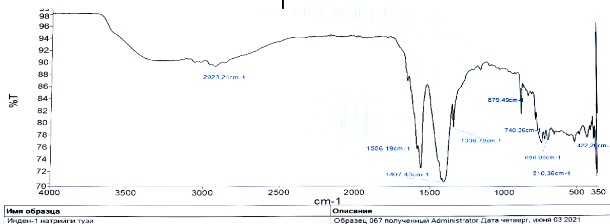
2-rasm. Inden-1 natriyli tuzining IQ-spektri
