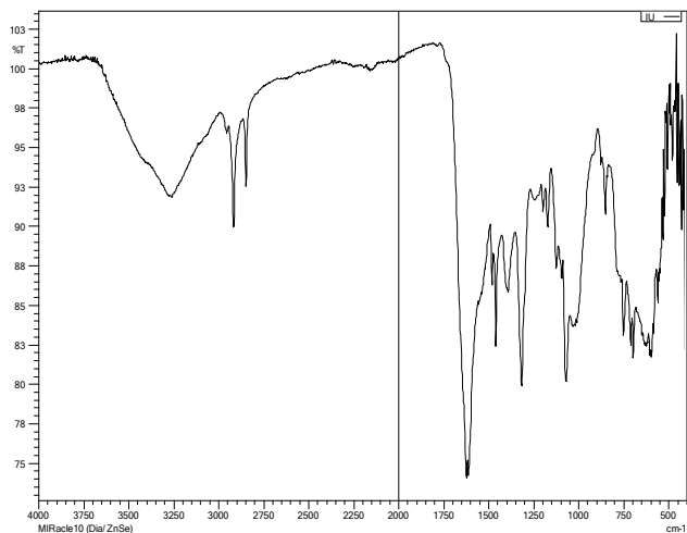
1-rasm. Toza indigoning IQ-spektri.
